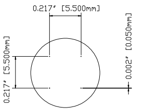
DETAIL B - DOT SPEC SCALE 5:1
