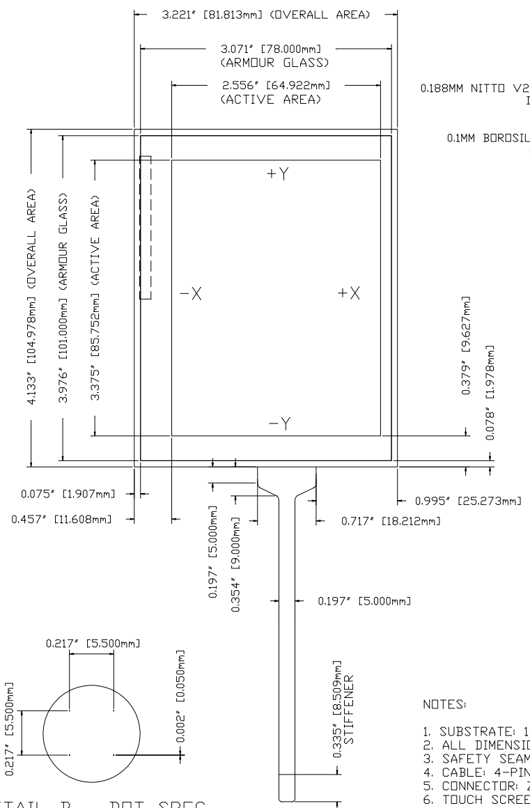
DETAIL B - DOT SPEC SCALE 5:1
