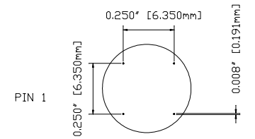
DETAIL A - DOT SPEC SCALE 5:1
